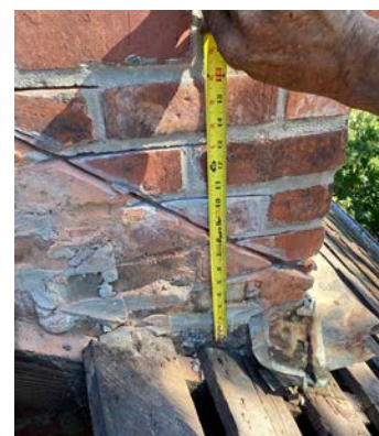
Fig. 2 If previous counter-flashing was set into a diagonal groove cut into bricks, this must be repaired with colour-matched mortar.
