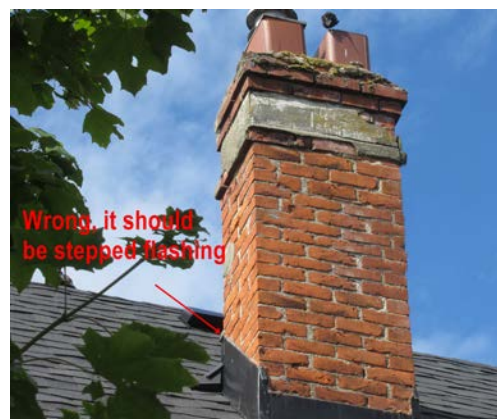
Fig. 3 Incorrect flashing.
