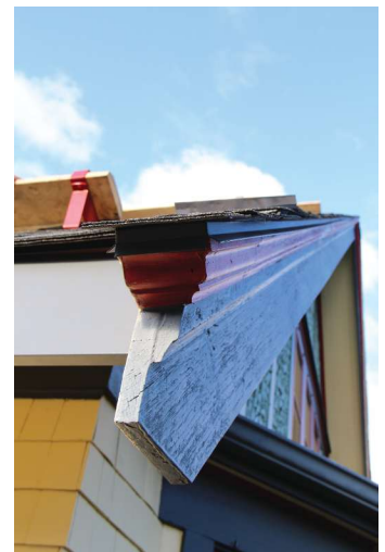
Fig. 5 Gable edge drip flashing
