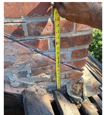
Fig. 3 If previous counter-flashing was set into a diagonal groove cut into bricks, this must be repaired with colour-matched mortar.
